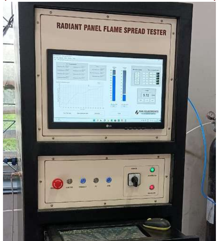
Inspection of Radiant Panel Flame Spread Tester at Fire Testing Laboratory, NFSC.
